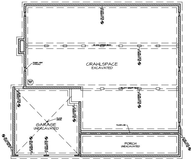
FOUNDATION PLAN A-4
